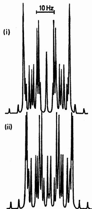
FIGURE 4 Computed ^1\text{H} n.m.r. spectra for \text{MePF}(\text{S})\cdot\text{S}\cdot\text{PF}(\text{S})\text{Me} , (IIIa). (i) Isomer A. (ii) Isomer B. The spectra are correctly offset to correspond to the observed spectrum (see Figure 2.)
