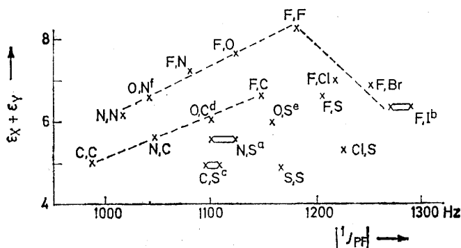
FIGURE 6 Plot of {}^1J_{\text{PF}} vs. \epsilon_X + \epsilon_Y for compounds of the type XYP(S)F, where \epsilon_X and \epsilon_Y are the Allred-Rochow electronegativities 24 of the \alpha -atom in substituents X and Y respectively. The data (where multivalent nuclei are concerned) are for substituents OMe, NMe 2 , Me, and SMe, except where indicated below. The values are taken from refs. 9, 15, 25–30. The dashed lines show correlations. (a) Ref. 27 gives values from {}^{19}\text{F} and {}^{31}\text{P} resonance which differ by 23 Hz. (b) Data from refs. 26 and 30 differ by 19 Hz. (c) Data are for X = Me, Y = SEt (1093 Hz, ref. 15) and X = Me, Y = SH (1107 Hz, ref. 9). (d) This value is for X = OEt, Y = Et (ref. 15). (e) This value is for X = OMe, Y = SEt (ref. 27). (f) This value is for X = OMe, Y = NH 2 (1042 Hz, ref. 29). Ref. 29 also gives J = 1123 Hz for X = OEt, Y = NH 2 but this is presumably in error. The above notes indicate that not all the literature values can be accurate, and caution is needed in discussing correlations
