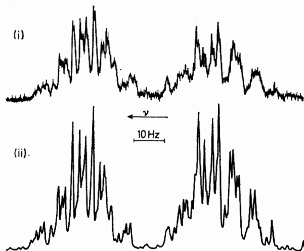
FIGURE 5 High frequency region of the 94.075 MHz ^{19}\text{F} spectrum for \text{MePF}(\text{S})\cdot\text{S}\cdot\text{PF}(\text{S})\text{Me} , (IIIa). The band due to isomer A is to high frequency of that due to isomer B. (i) Observed spectrum. (ii) Computed spectrum
